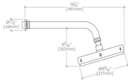
SIDE VIEW SCALE: 1/2"=1'-0"
